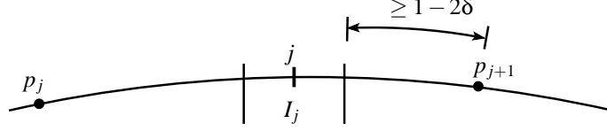
Figure 4: An example of a good server of left type. There are no servers between the position of server j ( p_j ) and I_j and the distance (to the right) of all the other servers from I_j is at least 1 - 2\delta .
