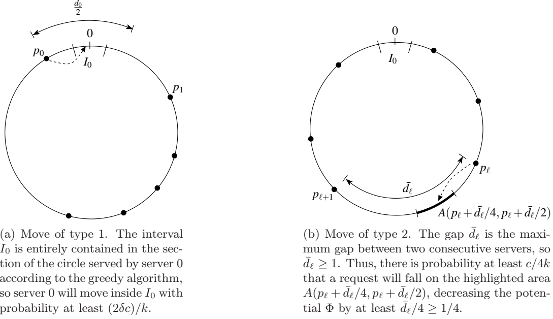
Figure 3: Examples of moves in Step 1.1
